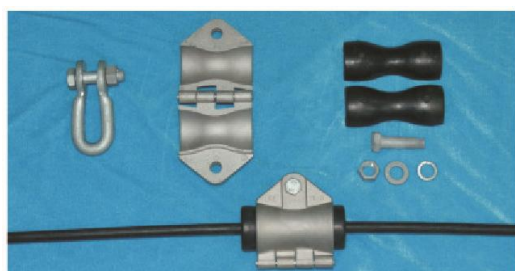
SAXD-100-XX suspension clamp
